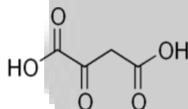
OXALOACETIC ACID
