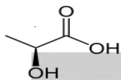
LACTIC ACID
