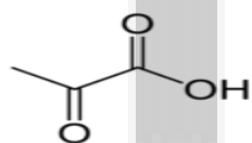
PYRUVIC ACID
